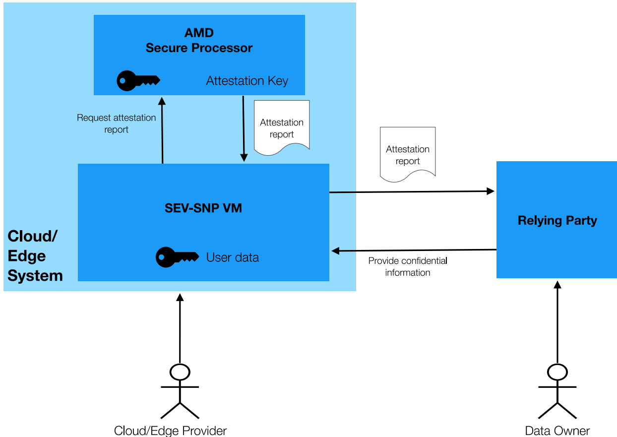
FIGURE 25: AMD REMOTE ATTESTATION
