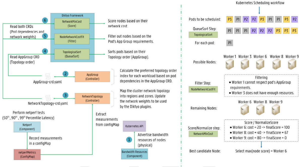
FIGURE 11: DIKTYO FRAMEWORK AND KUBERNETES SCHEDULING WORKFLOW
