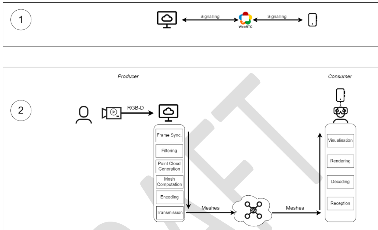
FIGURE 8: HOLOGRAPHIC COMMUNICATION
