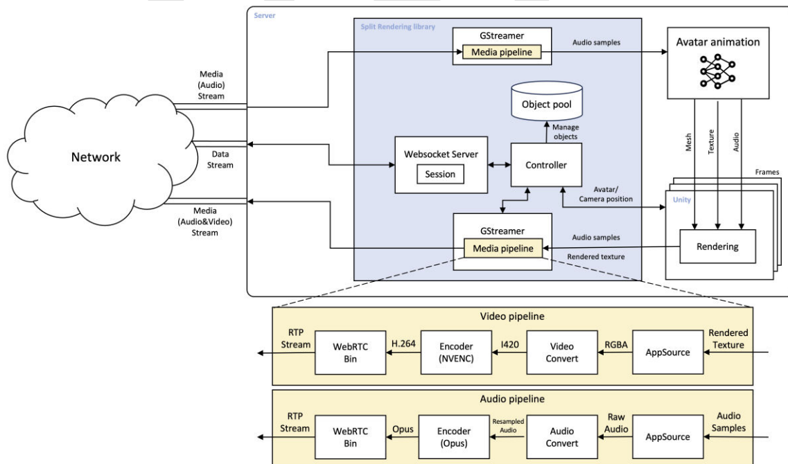
FIGURE 10: ARCHITECTURE OF THE SERVER APPLICATION OF THE PLATFORM FOR REAL-TIME ANIMATION AND STREAMING OF REALISTIC AVATARS
