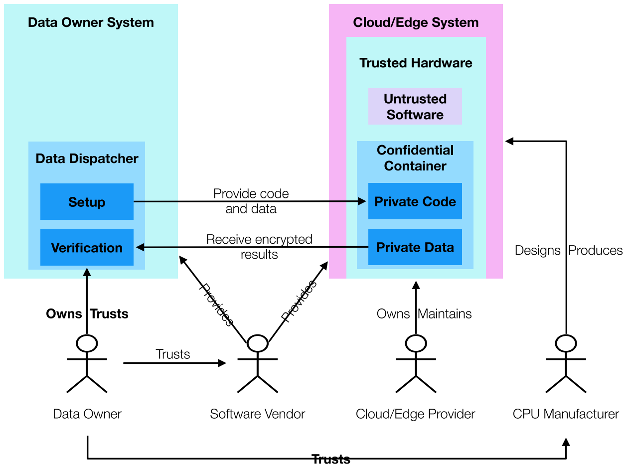
FIGURE 18: TRUST RELATIONSHIP IN CONFIDENTIAL COMPUTING
